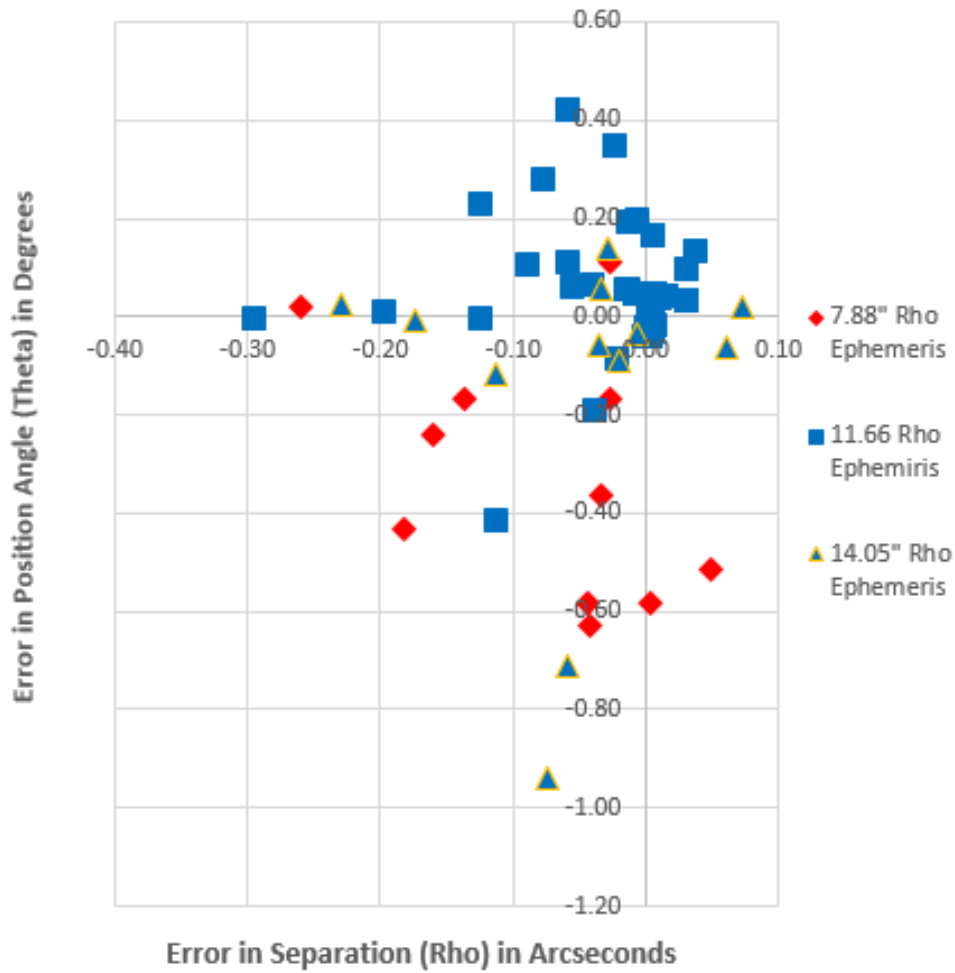
Figure 15. Plot of the impact of separation on the mean error for measurements taken with a green filter
