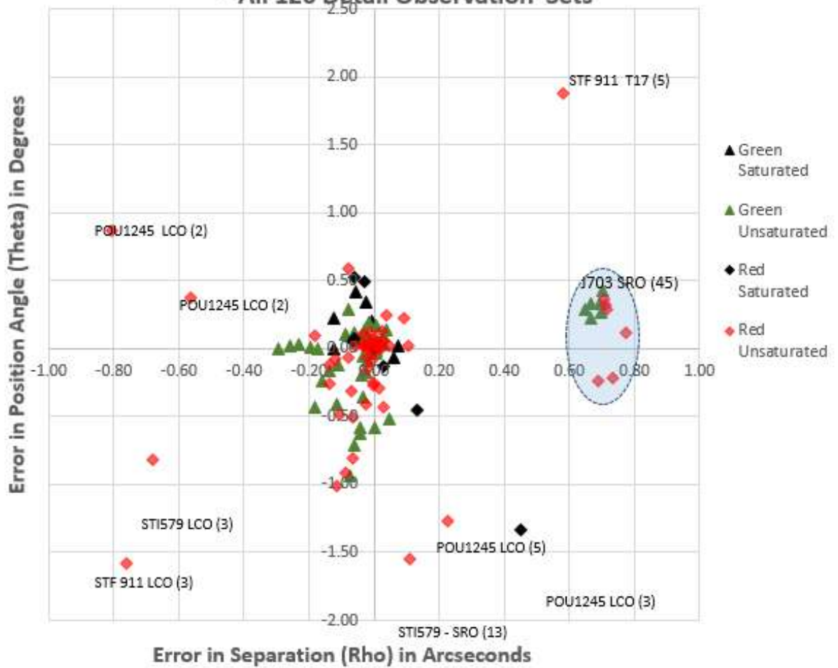
Figure 1. Plot of the mean error in position and separation for the 126 detail observation sets measurements coded by saturation and filter
